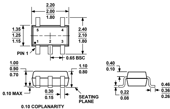
Figure 43. 5-Lead Thin Shrink Small Outline Transistor Package [SC70] (KS-5)
