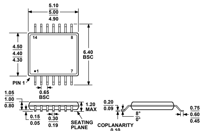
Figure 42. 14-Lead Thin Shrink Small Outline Package [TSSOP] (RU-14)
