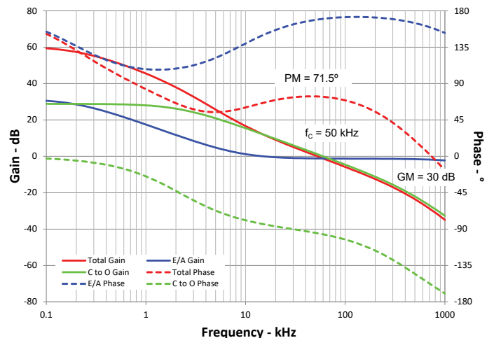
Figure 13: Bode Plot of the Complete System (red curve) R_Z = 8.25 \text{ k}\Omega , C_Z = 2.2 \text{ nF} , C_P = 10 \text{ pF} L_O = 10 \text{ }\mu\text{H} , C_O = 2 \times 10 \text{ }\mu\text{F} Ceramic
