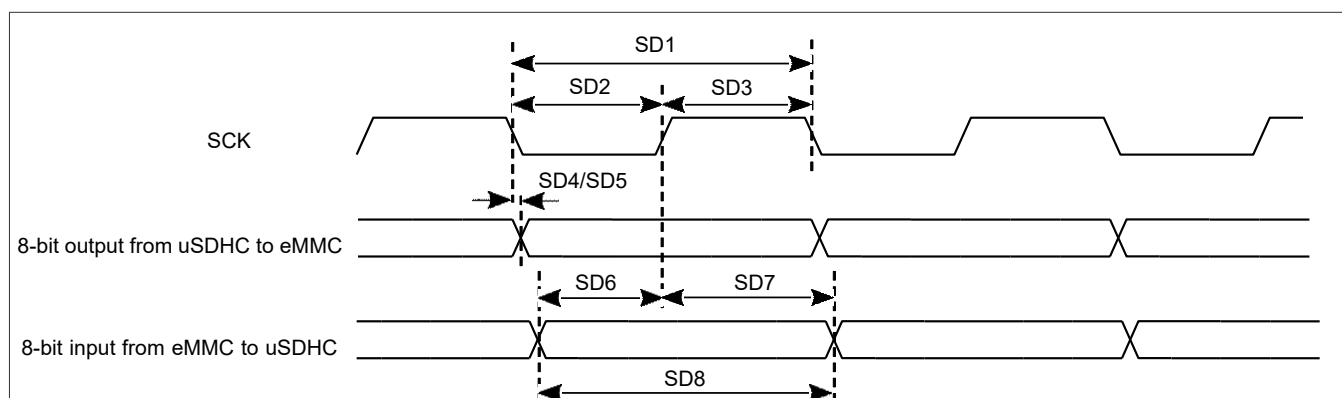
Figure 26. SDR50/SDR104 timing
