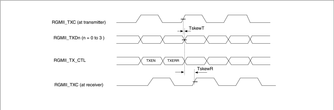
Figure 29. RGMII transmit signal timing diagram original
