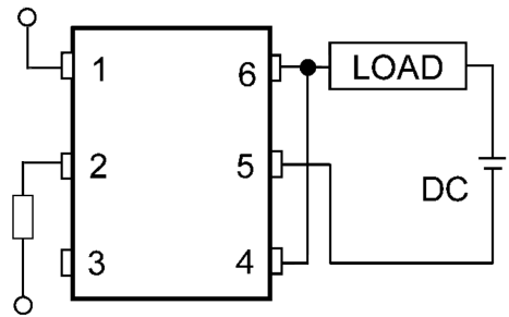
Fig. 12.2.3 C Connection
