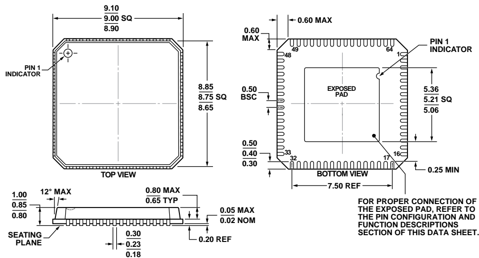
Figure 60. 64-Lead Lead Frame Chip Scale Package [LFCSP_VQ] 9 mm x 9 mm Body, Very Thin Quad (CP-64-7) Dimensions shown in millimeters
