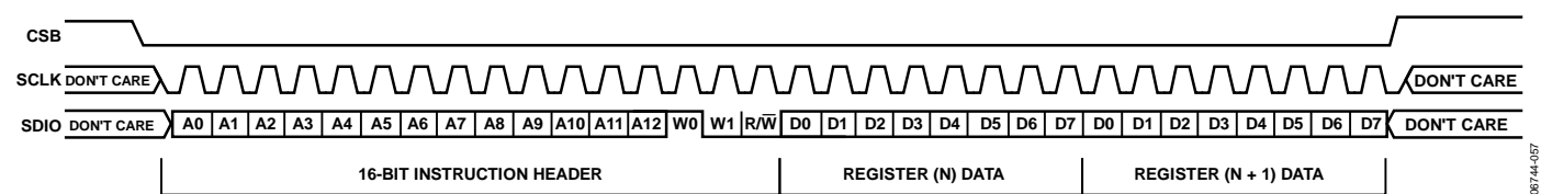
Figure 57. Serial Control Port Write—LSB First, 16-Bit Instruction, Two Bytes Data
