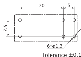
Recommended PC board pattern ( BOTTOM VIEW )
