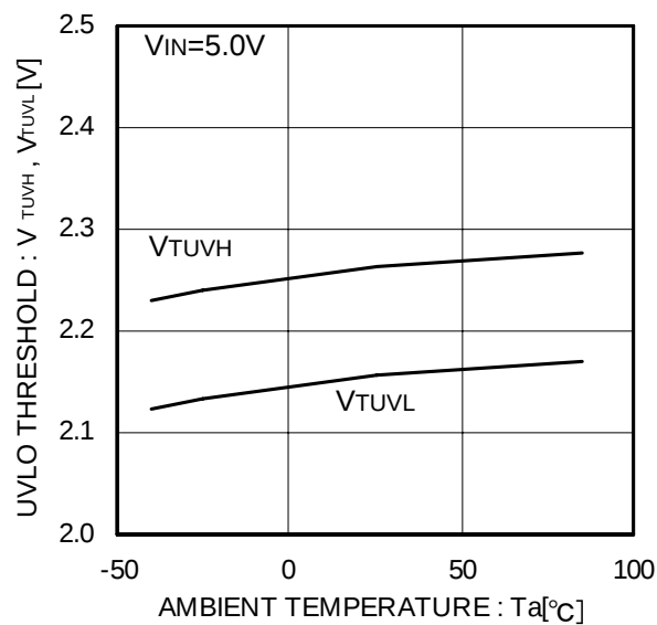
Figure 16. UVLO threshold
