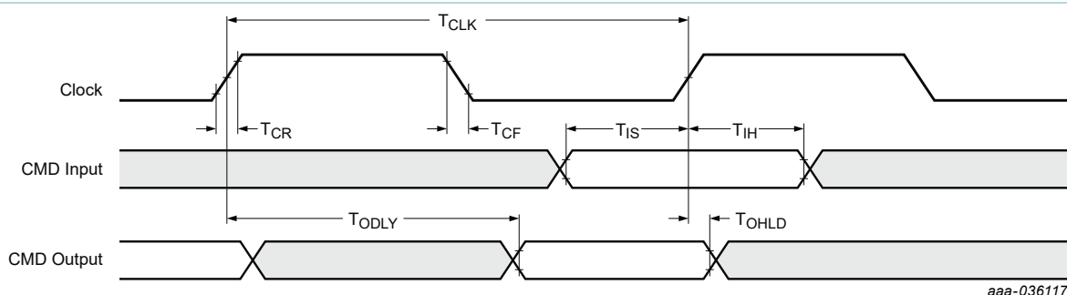
Figure 17. SDIO CMD timing diagram—DDR50 mode (50 MHz)
