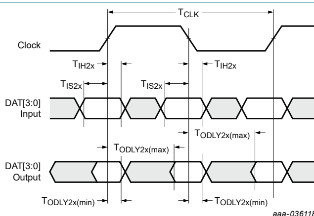
Figure 18. SDIO DAT[3:0] timing diagram—DDR50 mode [1] (50 MHz)
