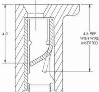
SECTION X-X
