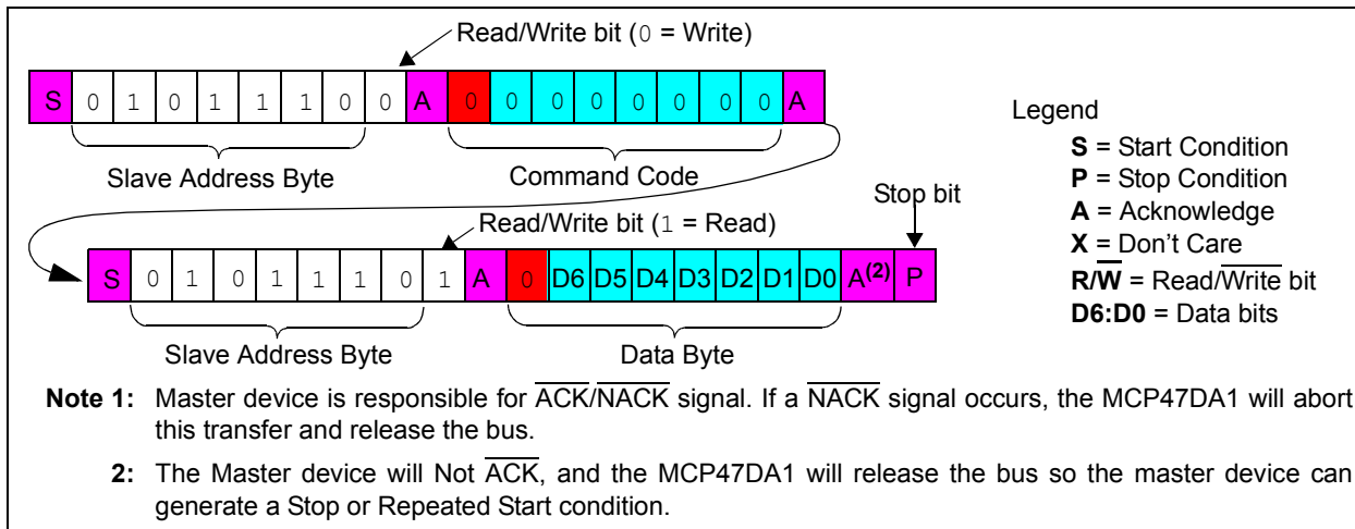
FIGURE 5-14: I 2 C Read Command Format.
