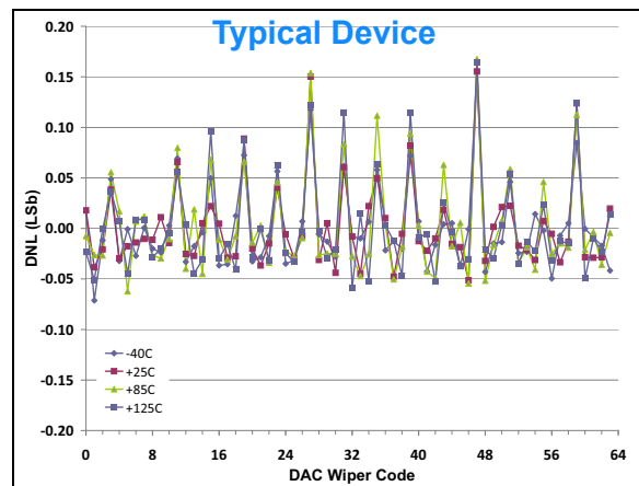
FIGURE 2-17: DNL vs. Code and Temperature. V_{DD} = 3.6\text{V} , V_{REF} = 1.0\text{V}
