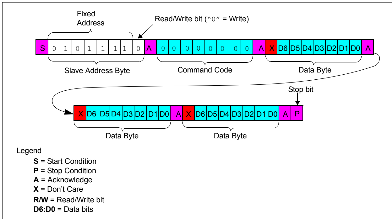
FIGURE 5-12: I²C Write Command Format.
