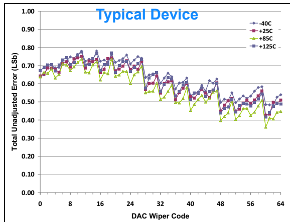
FIGURE 2-55: Total Unadjusted Error vs. Code and Temperature.
