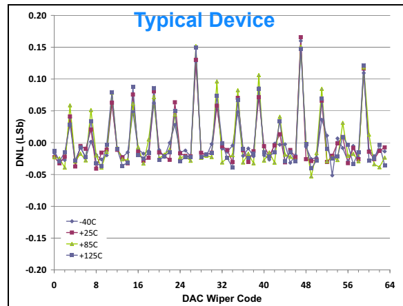
FIGURE 2-16: DNL vs. Code and Temperature. V_{DD} = 3.6\text{V} , V_{REF} = 1.65\text{V}
