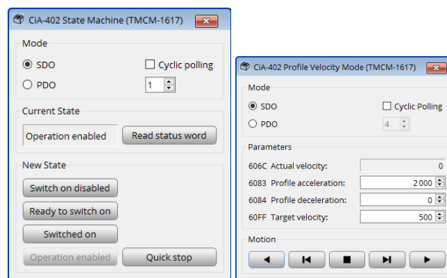
Figure 8: Enter Operation Enabled State and use the Profile Velocity Mode
