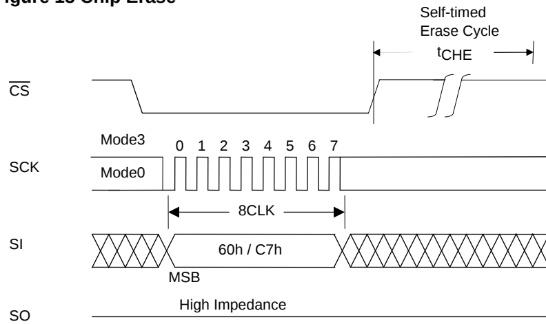
Figure 13 Chip Erase
