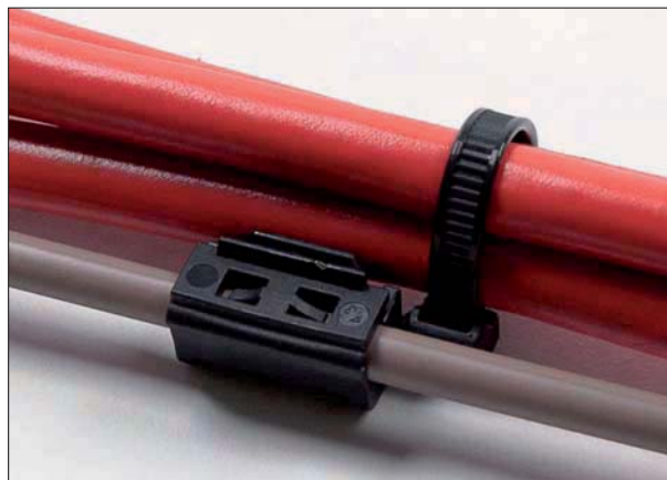
T50SOSWA - the easy way for parallel guidance of cables next to a wire.
