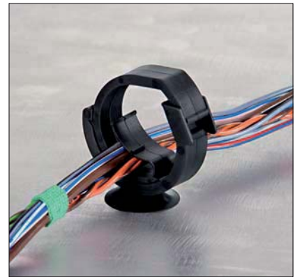
Automatic Harness Clip closed.
