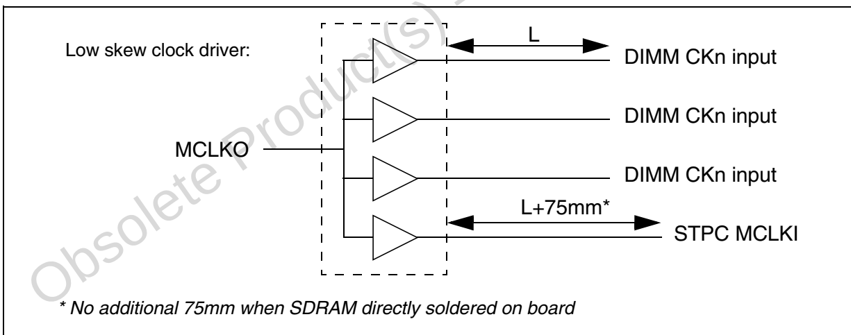
Figure 6-20. Clock Routing
