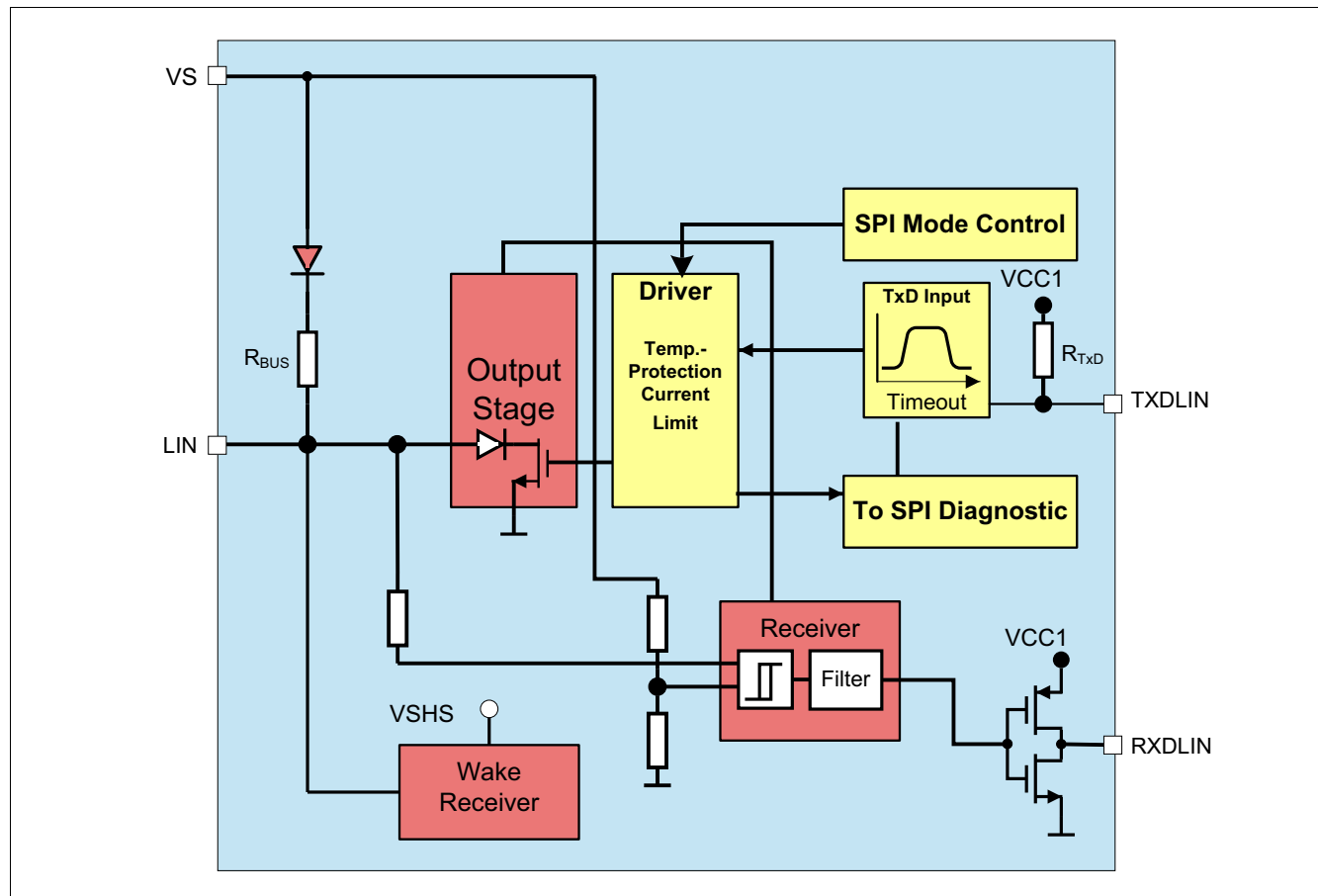
Figure 24 Block Diagram
