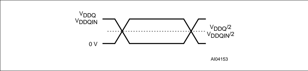
Figure 6. AC measurement input/output waveform
