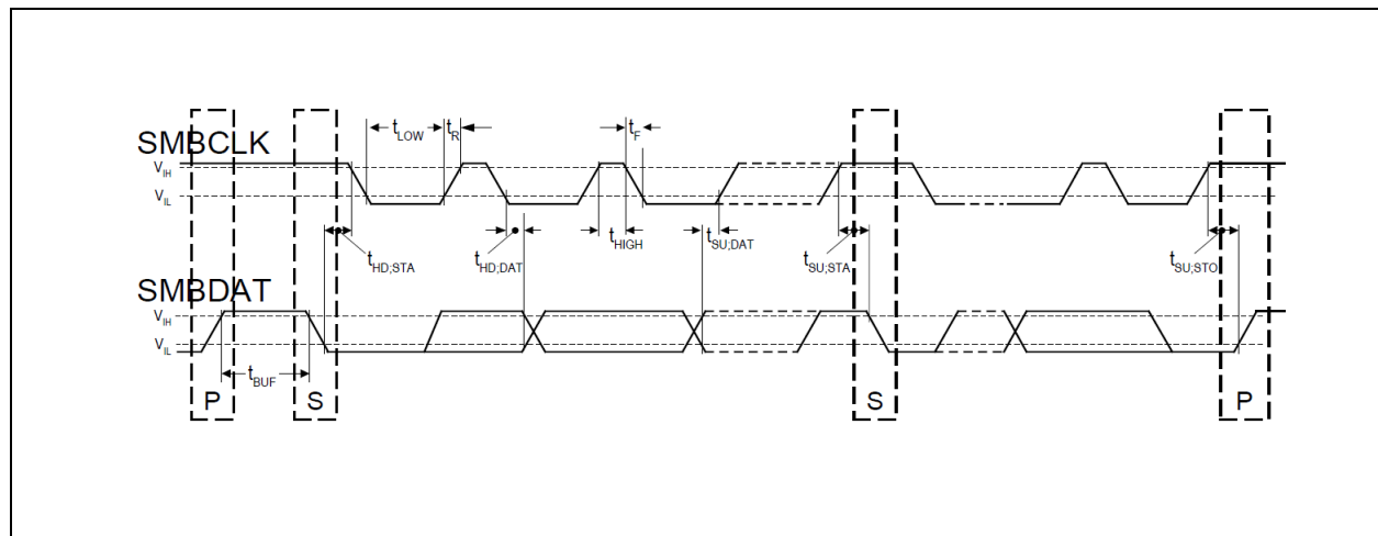
Figure 24. SMBus Timing
