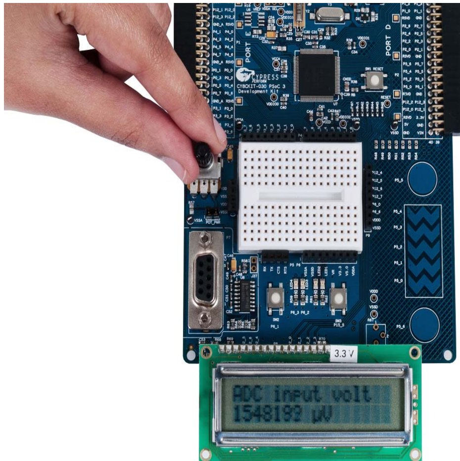
Figure 5-3. Voltage Display
