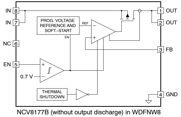
Figure 2. Internal Block Diagram
