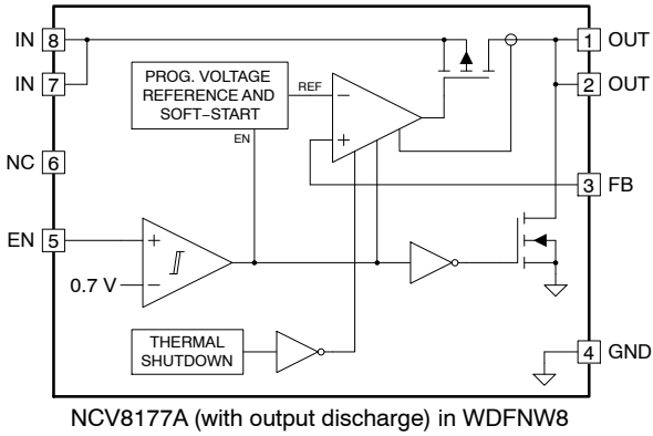
Figure 2. Internal Block Diagram
