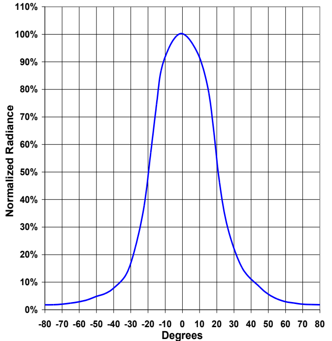
Beam Angle
