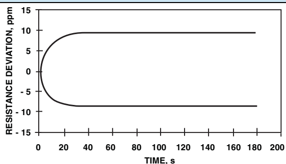
FIGURE 2 - RAPID STABILIZATION
