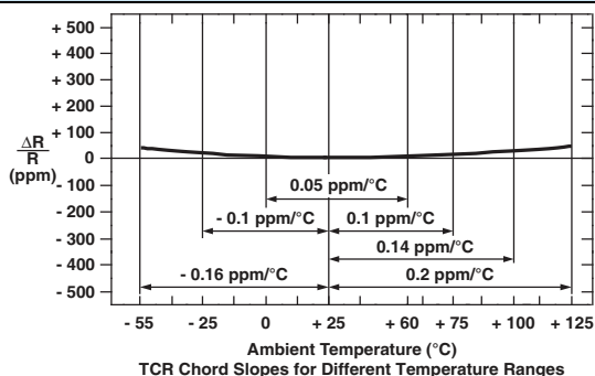
FIGURE 4 - TYPICAL RESISTANCE/TEMPERATURE CURVE (Z-FOIL)
