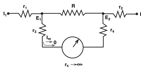
FIGURE 6 - KELVIN CONNECTION
