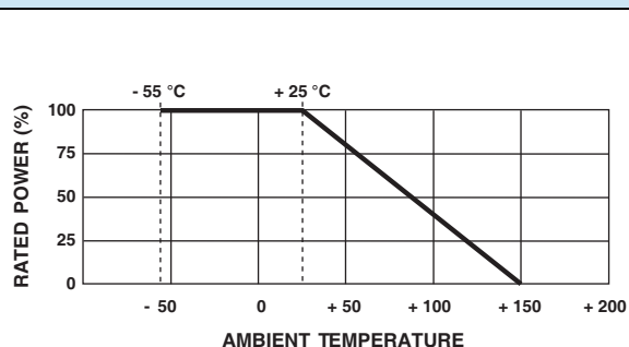
FIGURE 5 - POWER DERATING CURVE
