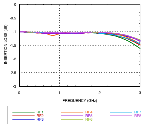
Insertion Loss
