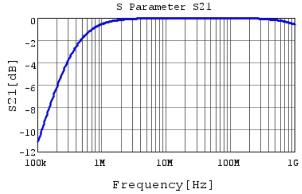
RDER73A472K2M1H03A S21 DCOV, 25degC
