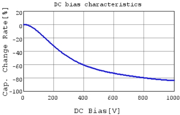
RDER73A472K2M1H03A C-DC bias capchange, 25.0
