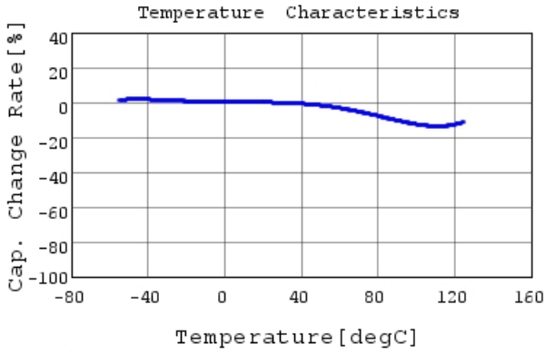
RDER73A472K2M1H03A C-Temp. capchange, DCOV,
