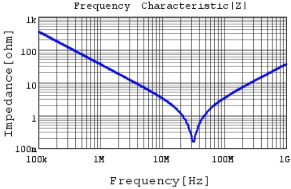
RDER73A472K2M1H03A |Z| DCOV, 25degC
