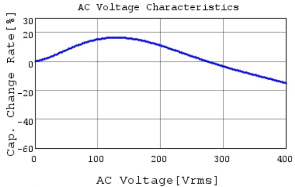
RDER73A472K2M1H03A C-AC Voltage capchange, I
