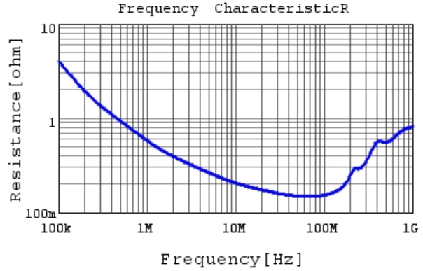
RDER73A472K2M1H03A R DCOV, 25degC
