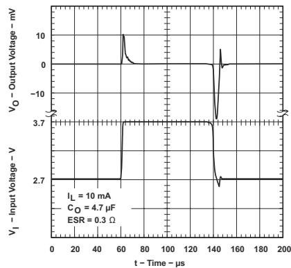
Figure 5-37. TPS76915 Line Transient Response (Legacy Chip)
