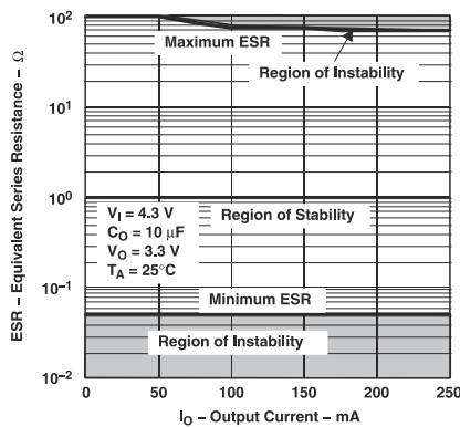
Figure 5-54. Typical Region of Stability ESR vs Output Current (New Chip)
