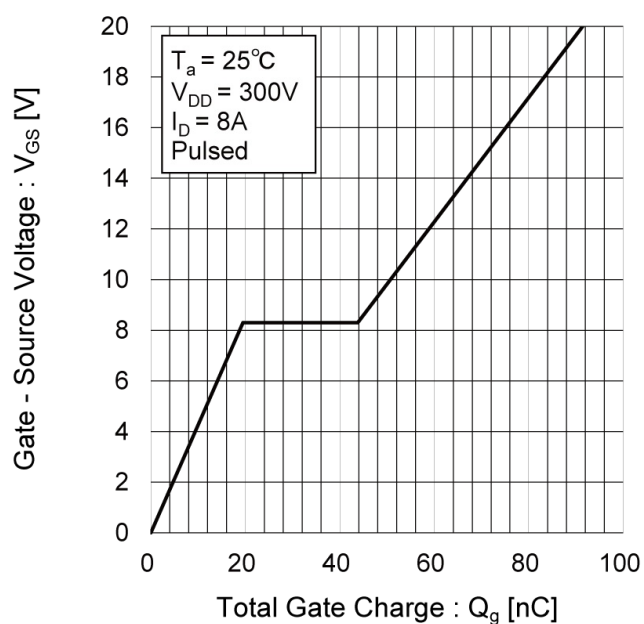
Fig.16 Gate Charge
