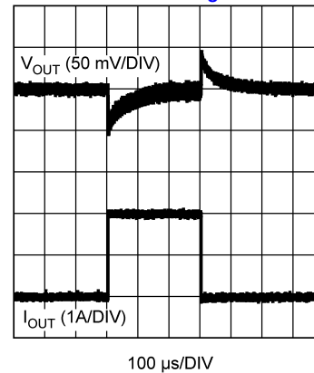
Load Transient V_{OUT} = 3.3V , I_{OUT} = 100\text{ mA} - 2A @ slewrate = 2A / \mu s Refer to Figure 46
