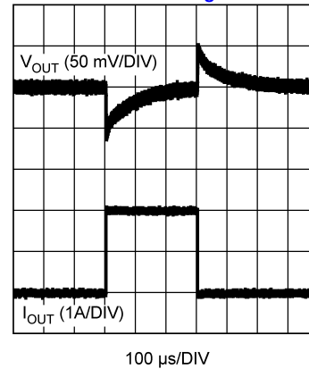
Load Transient V_{OUT} = 5V , I_{OUT} = 100\text{ mA} - 2A @ slewrate = 2A / \mu s Refer to Figure 40
