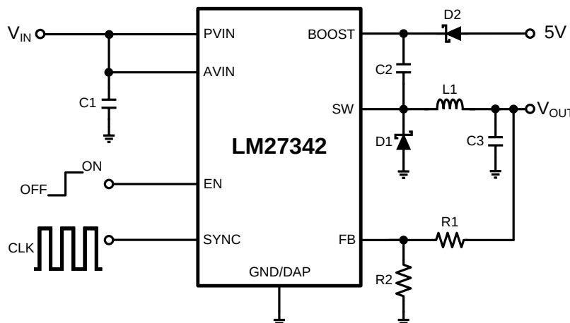
Figure 33. External Diode Charges C_{\text{BOOST}}
