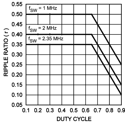
Figure 36. Recommended Ripple Ratio Vs. Duty Cycle
