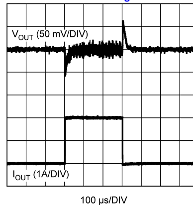
Load Transient V_{OUT} = 1.8V , I_{OUT} = 100\text{ mA} - 2A @ slewrate = 2A / \mu s Refer to Figure 55
