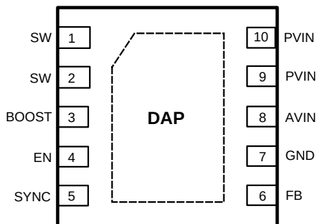
Figure 3. 10-Lead SON (Top View) See DSC0010A Package
