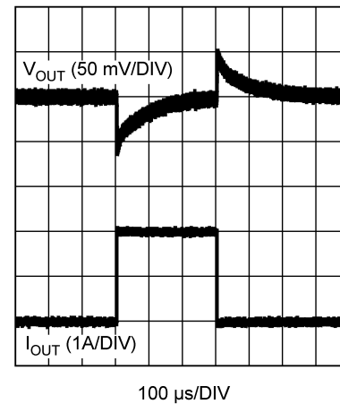
Figure 42. Transient Response I_{OUT} = 100\text{ mA} - 2\text{ A} @ slewrate = 2\text{ A} / \mu\text{s}
