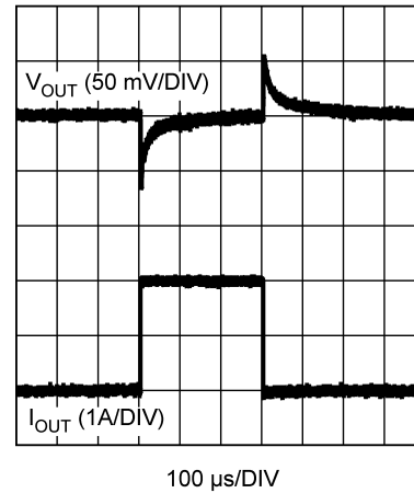
Figure 54. Transient Response I_{OUT} = 100\text{ mA} - 2\text{ A} @ slewrate = 2\text{ A} / \mu\text{s}
