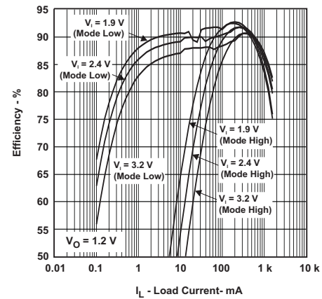
Figure 13. Efficiency vs Load Current, V_{OUT} = 1.2\text{ V}
