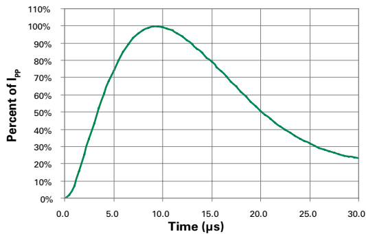
8/20μs Pulse Waveform
