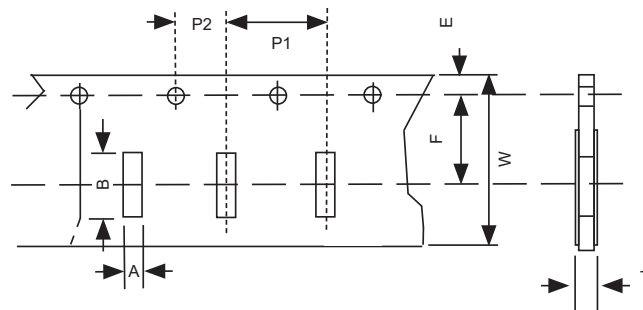
FIGURE 2 PAPER CARRIER
