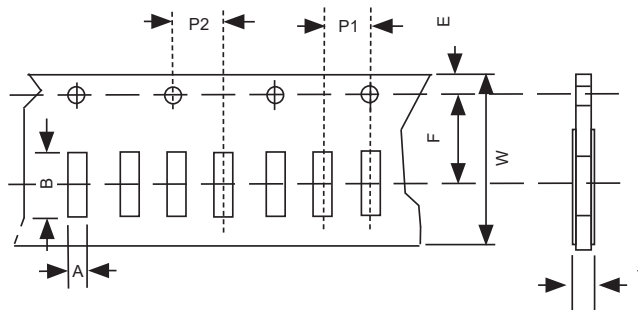
FIGURE 2 PAPER CARRIER
