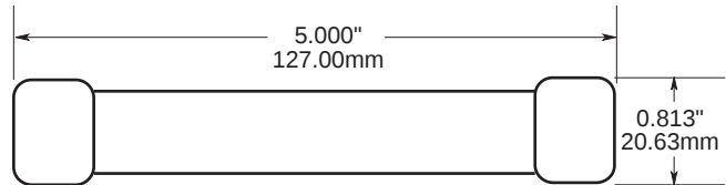
Dimensions - inches (mm)
