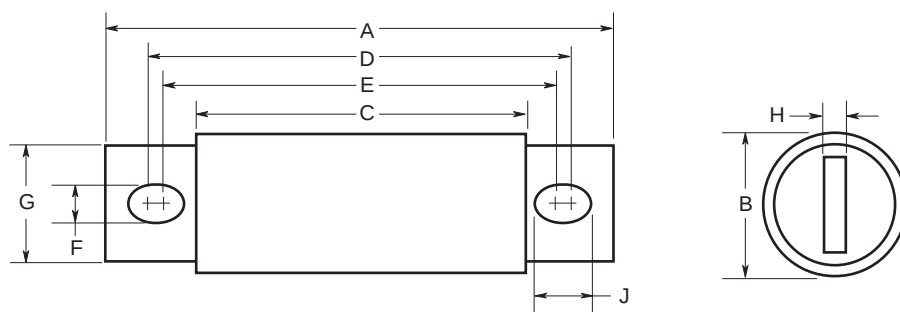
Figure 1: 35 – 800A Range
