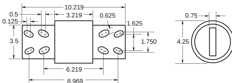
Figure 2: 1400 – 1600A Range
