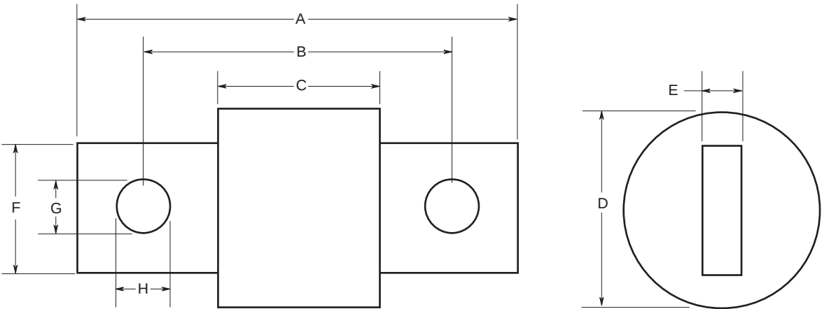
Figure 3: 500 – 1000A Range
