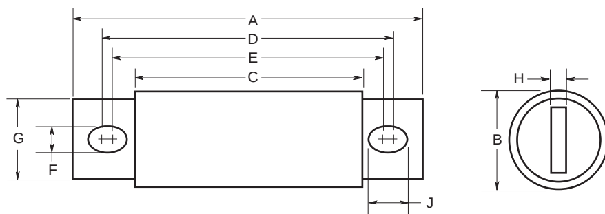
Figure 1: 35 – 800A Range
