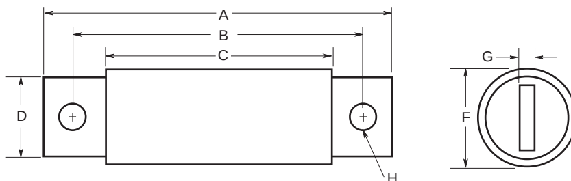
Figure 2: 70 – 600A Range
