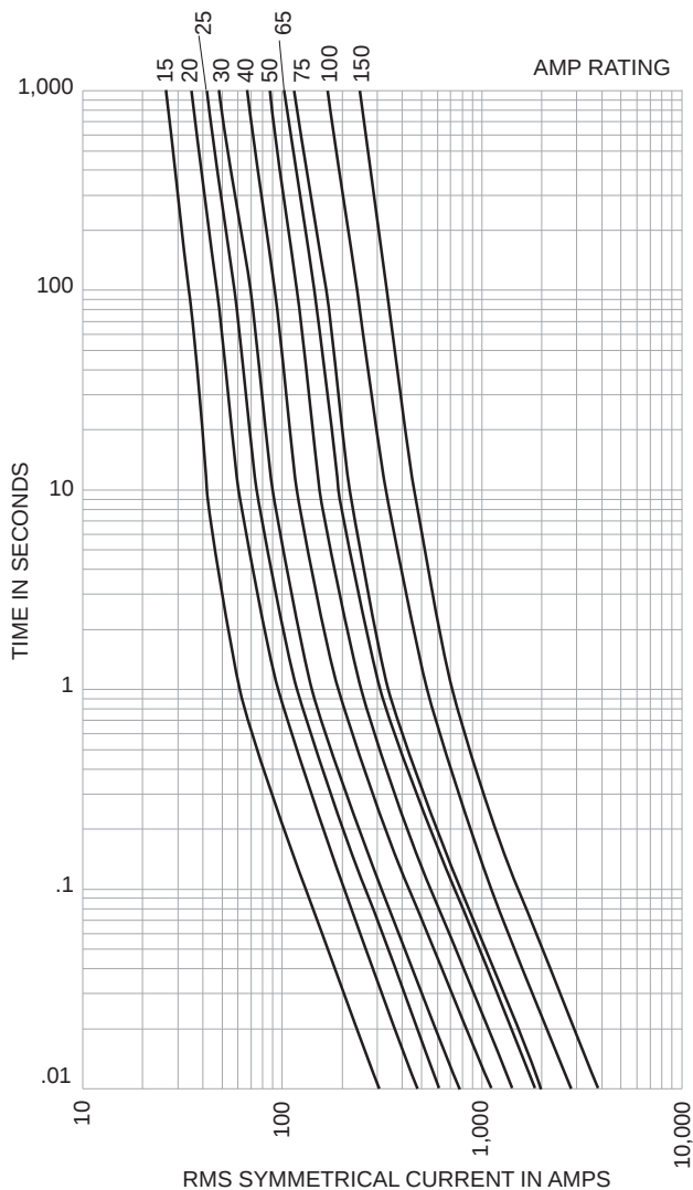
Time-Current Characteristics – Min. Melt
