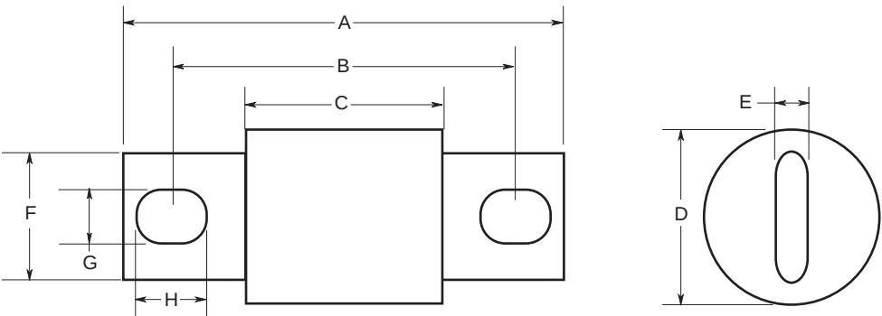
Figure 2: 70 – 400A Range
