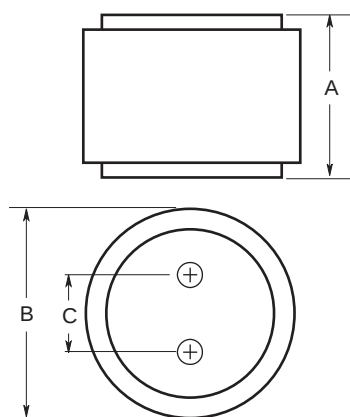
Figure 2: 1000 – 1200A Range
