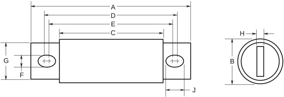
Figure 1: 40 – 800A Range
