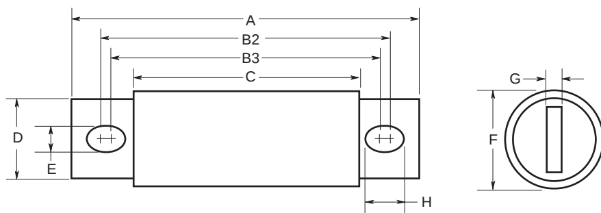
Figure 2: 35 – 200A Range
