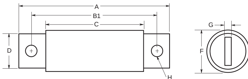
Figure 1: 4 – 30A &amp; 225 – 1000A Range
