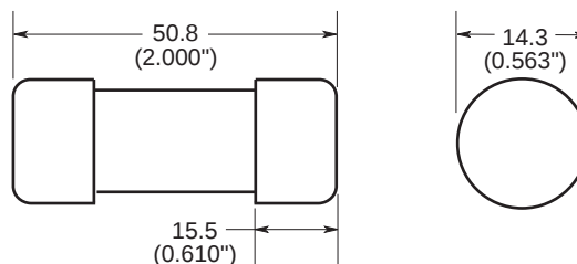
Dimensions - inches (mm)
