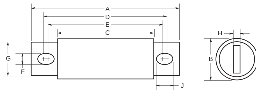
Figure 1: 35 – 1200A Range
