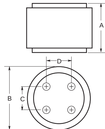
Figure 3: 1500 – 2500A Range
