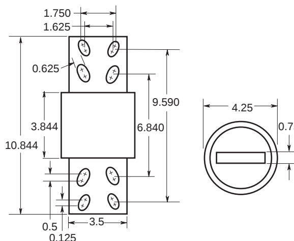
Figure 3: 1200A Range
