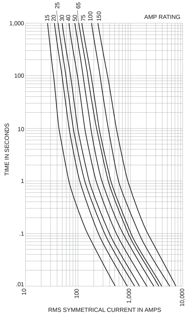
Time-Current Characteristics –Total Melting
