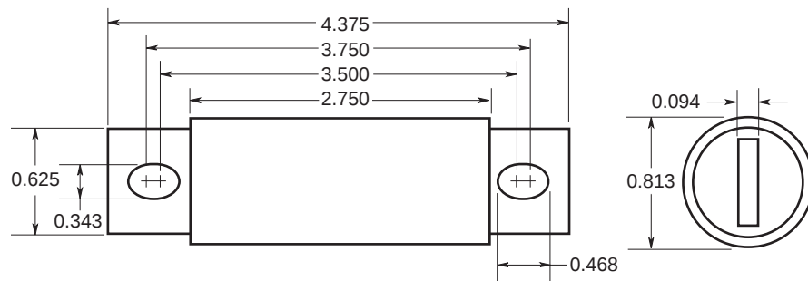
Figure 1: 35 – 60A Range
