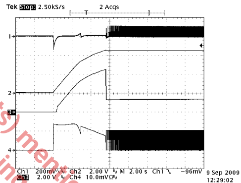
Fig. 14: 200mA Torch Mode with 0.55F Supercap, CH1 = V_{IN} , CH2 = V_{OUT} , CH3 = I_{LED} , CH4 = I_{VIN} = 0.5A/div
