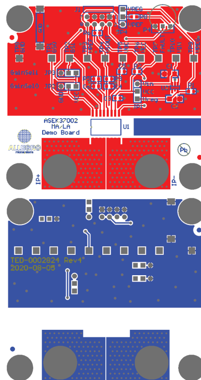
Figure 21: Top and Bottom Layers of ASEK37002 Evaluation Board
