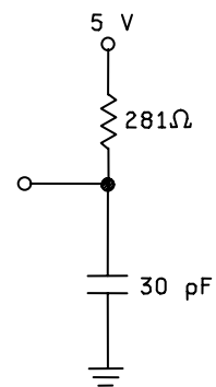
CIRCUIT C OUTPUT LOAD
