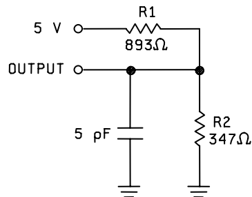
CIRCUIT B OUTPUT LOAD
