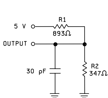
CIRCUIT A OUTPUT LOAD
