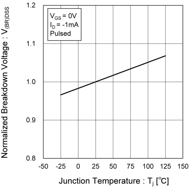
Fig.7 Normalized Breakdown Voltage vs. Junction Temperature
