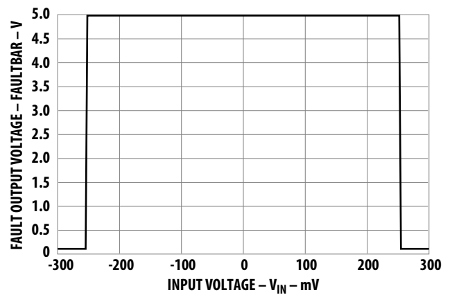
Figure 10. \overline{\text{FAULT}} output voltage vs. V_{IN}
