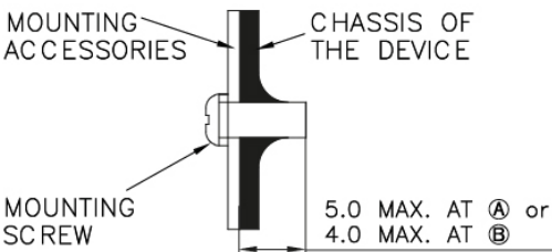
Fig. 4 Assembly Reference
