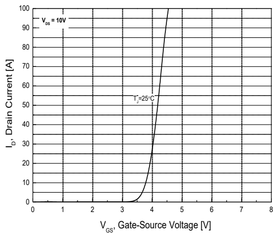
Fig.5 Transfer Characteristics
