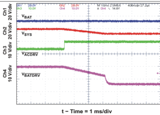
Figure 19. System Selector On Adapter Insertion With 390 \mu F SYS-to-PGND System Capacitor
