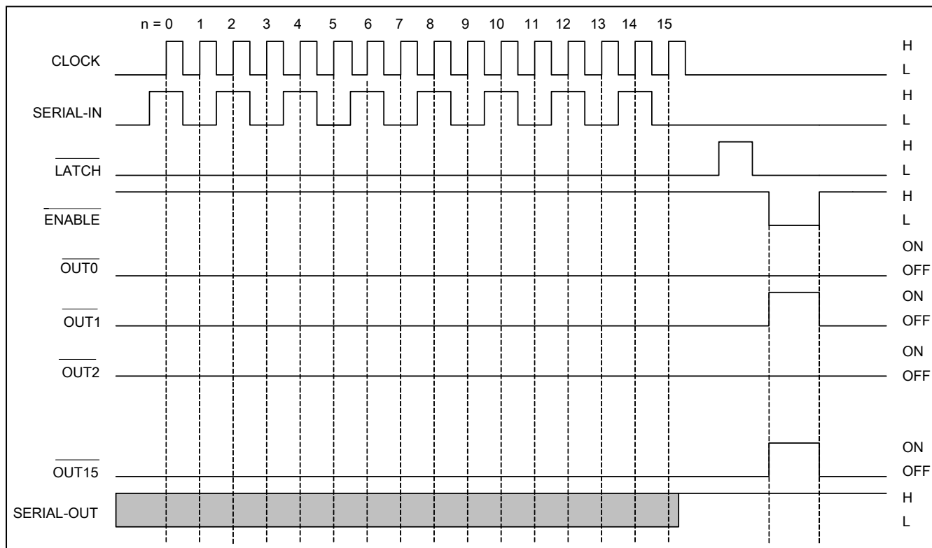
Figure 3 Timing Diagram
