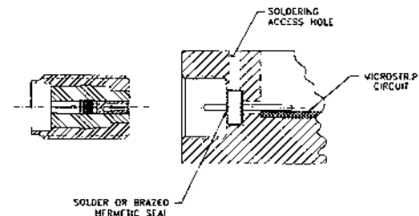
Drop-in Assembly - Feedthru Connector
