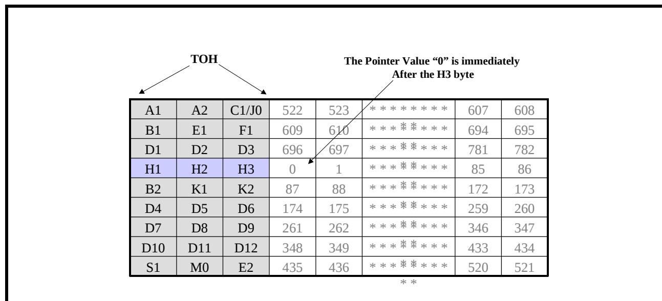
FIGURE 52. THE RELATIONSHIP BETWEEN THE CONTENTS OF THE "POINTER BITS" (E.G., THE 10-BIT EXPRESSION WITHIN THE H1 AND H2 BYTES) AND THE LOCATION OF THE J1 BYTE WITHIN THE ENVELOPE CAPACITY OF AN STS-1 FRAME
