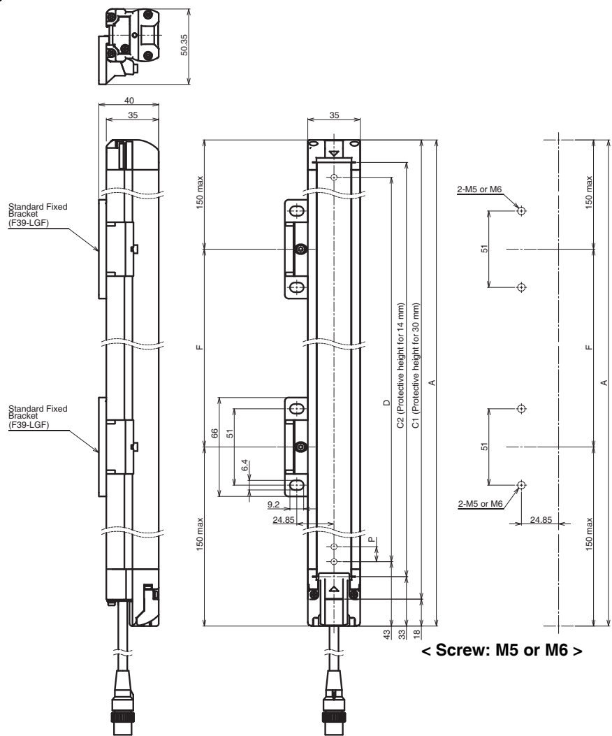
F3SG-□RA□□□□-30 Series
