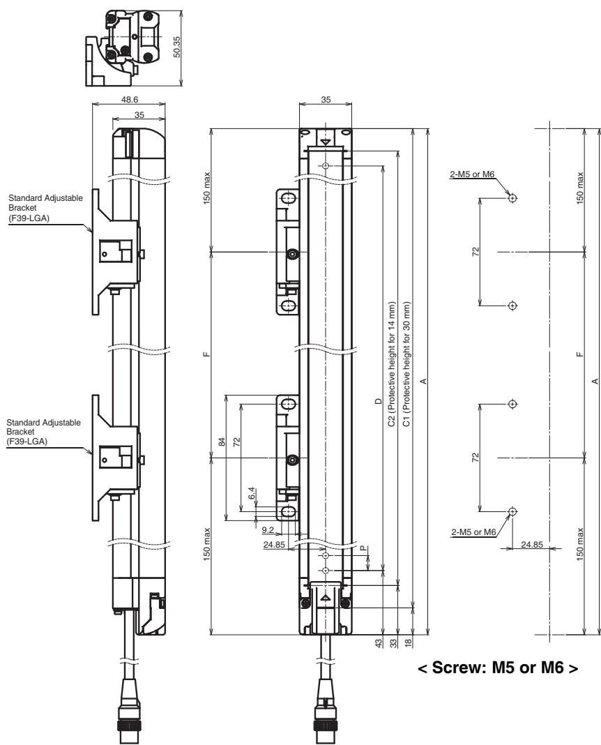
F3SG-□RA□□□□-30 Series
