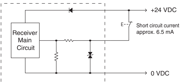
<PNP Output>
