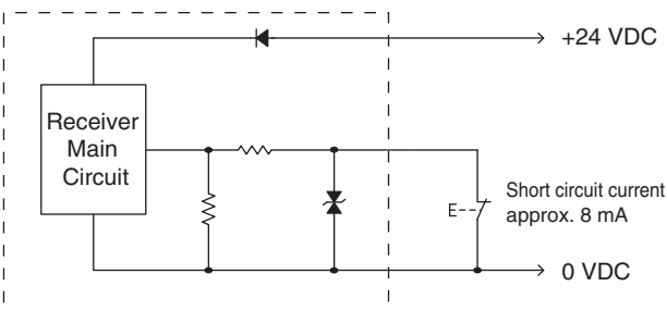
<NPN Output>
