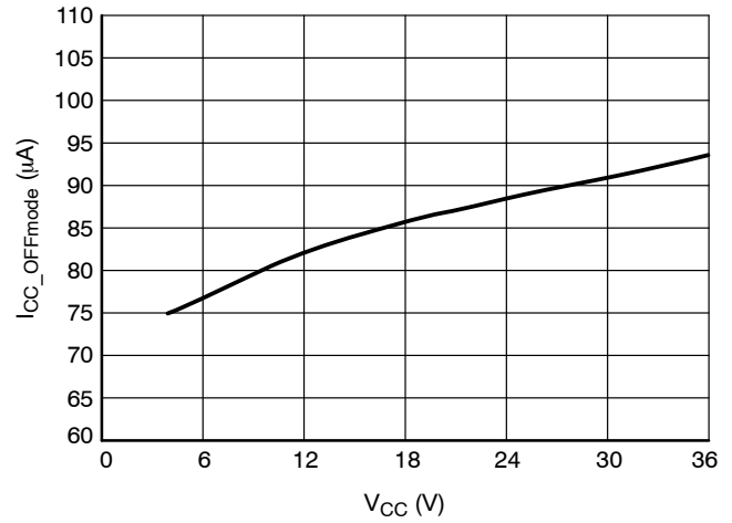
Figure 17. I_{CC} in OFF Mode at T_J = 25^{\circ}C , V_{SNS} < V_{SNSBIAS TH} , for NCP4355B
