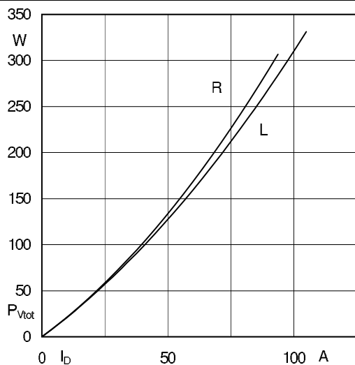
Fig. 3L: Max. power dissipation of two modules vs. direct current
