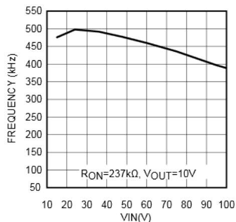
Figure 8-3. Frequency versus Input Voltage
