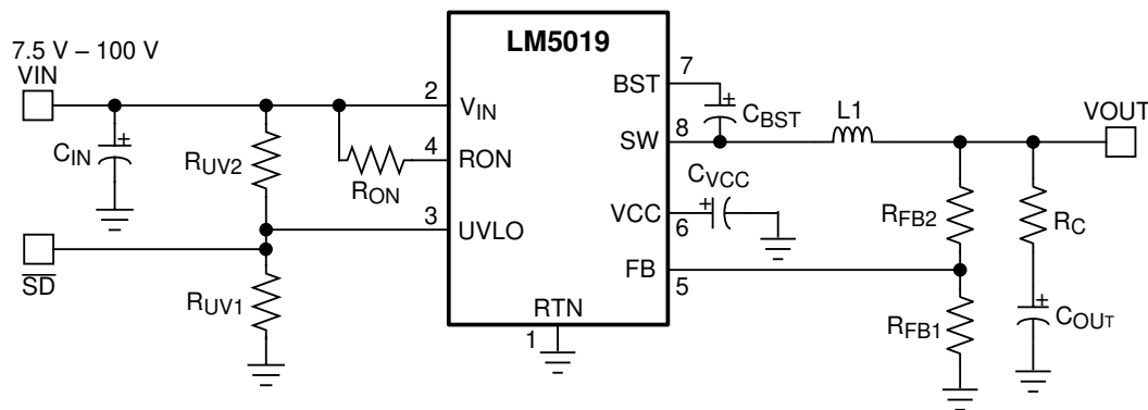
Typical Application
