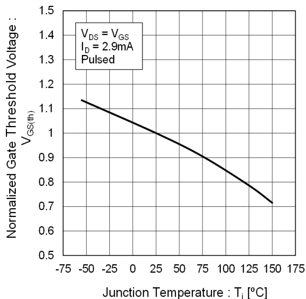
Fig.10 Normalized Gate Threshold Voltage vs. Junction Temperature
