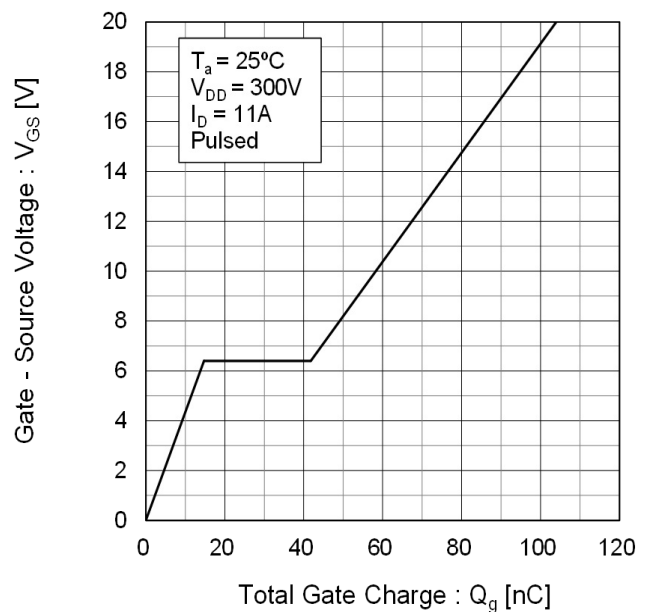
Fig.16 Gate Charge
