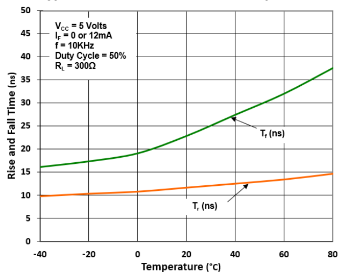
Typical Rise and Fall Time vs Temperature
