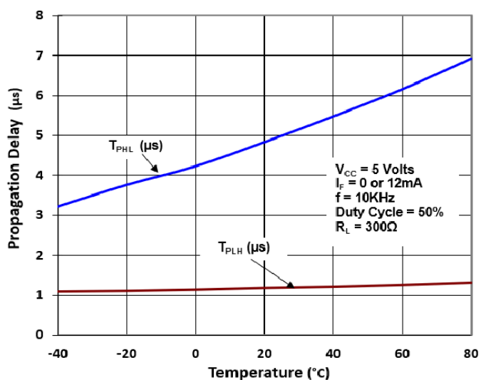
Typical Propagation Delay vs Temperature
