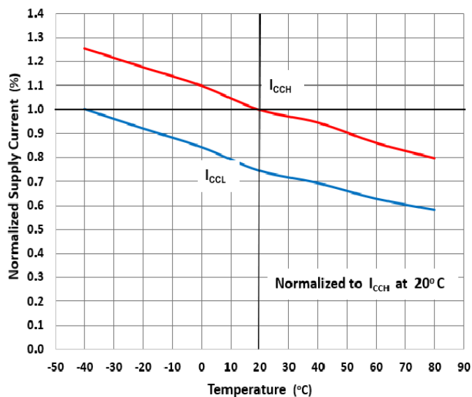
Supply Current vs Temperature
