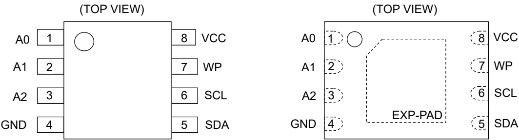
Figure 3-(a). Pin Configuration (SOP8, SOP-J8, TSSOP-B8, MSOP8) Figure 3-(b). Pin Configuration (VSON008X2030)
