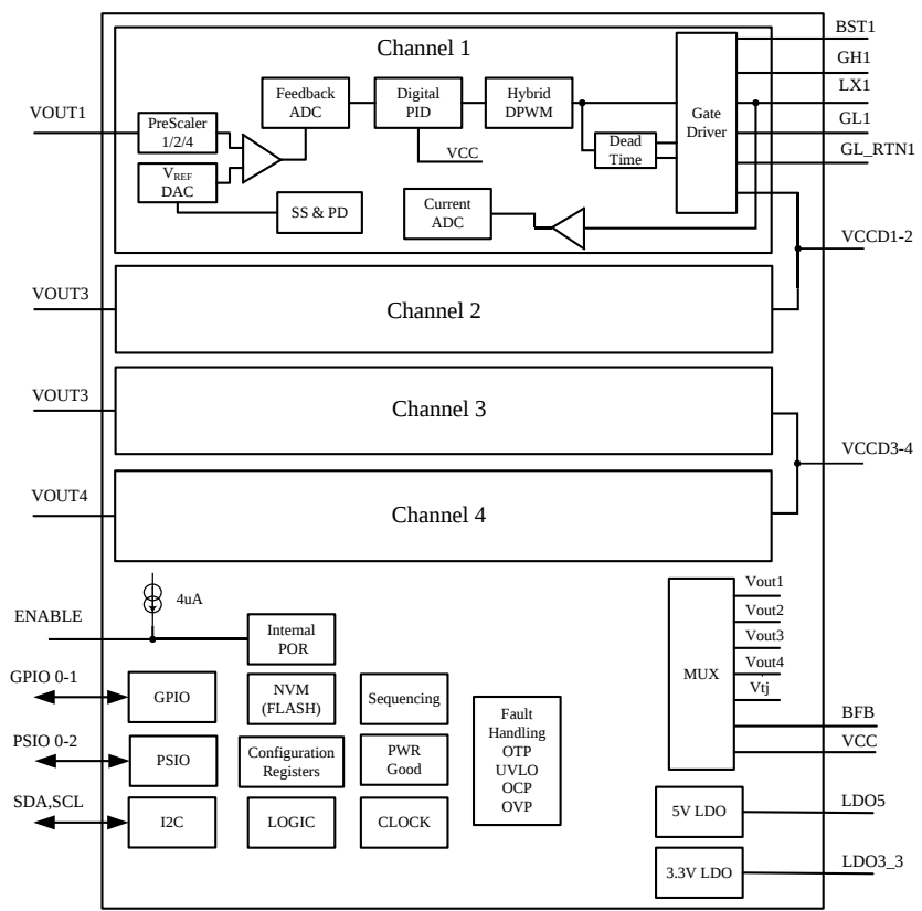
Fig. 2: XRP7724 Block Diagram
