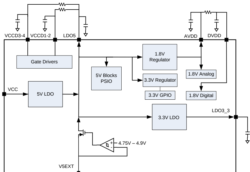
Fig. 3: XRP7724 LDO Block Diagram
