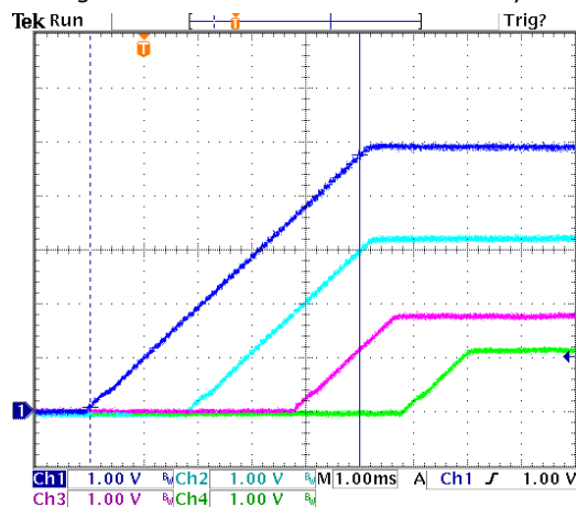
Fig. 9 Sequential Start-up
