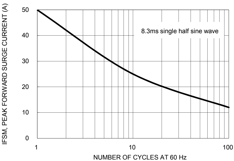
FIG. 2 MAXIMUM NON-REPETITIVE FORWARD SURGE CURRENT UNIDIRECTIONAL ONLY
